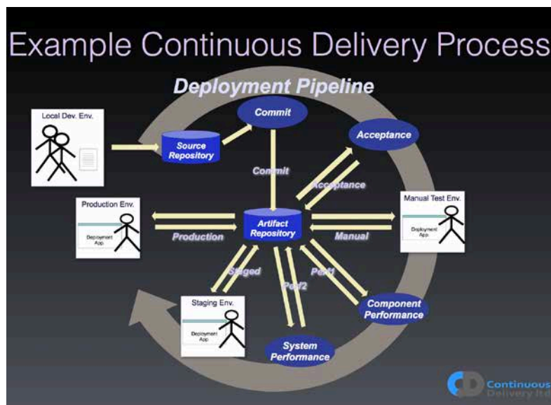
Image 13: Artifact repositories play a central role in deployment pipeline. Source: Dave Farley, Continuous Delivery Ltd. 2015. Slides at: http://bit.ly/1C9y7X8
