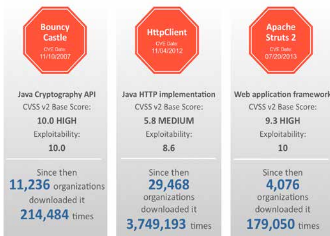
Image 8: Organizations continue to use known vulnerable components years after alerts have been issued. Source: Sonatype.
